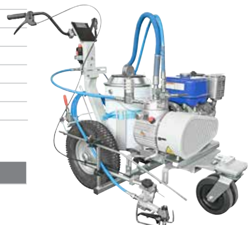
Part No. LA18383 DALÌ PLUS airless line striper with 23 l paint can
