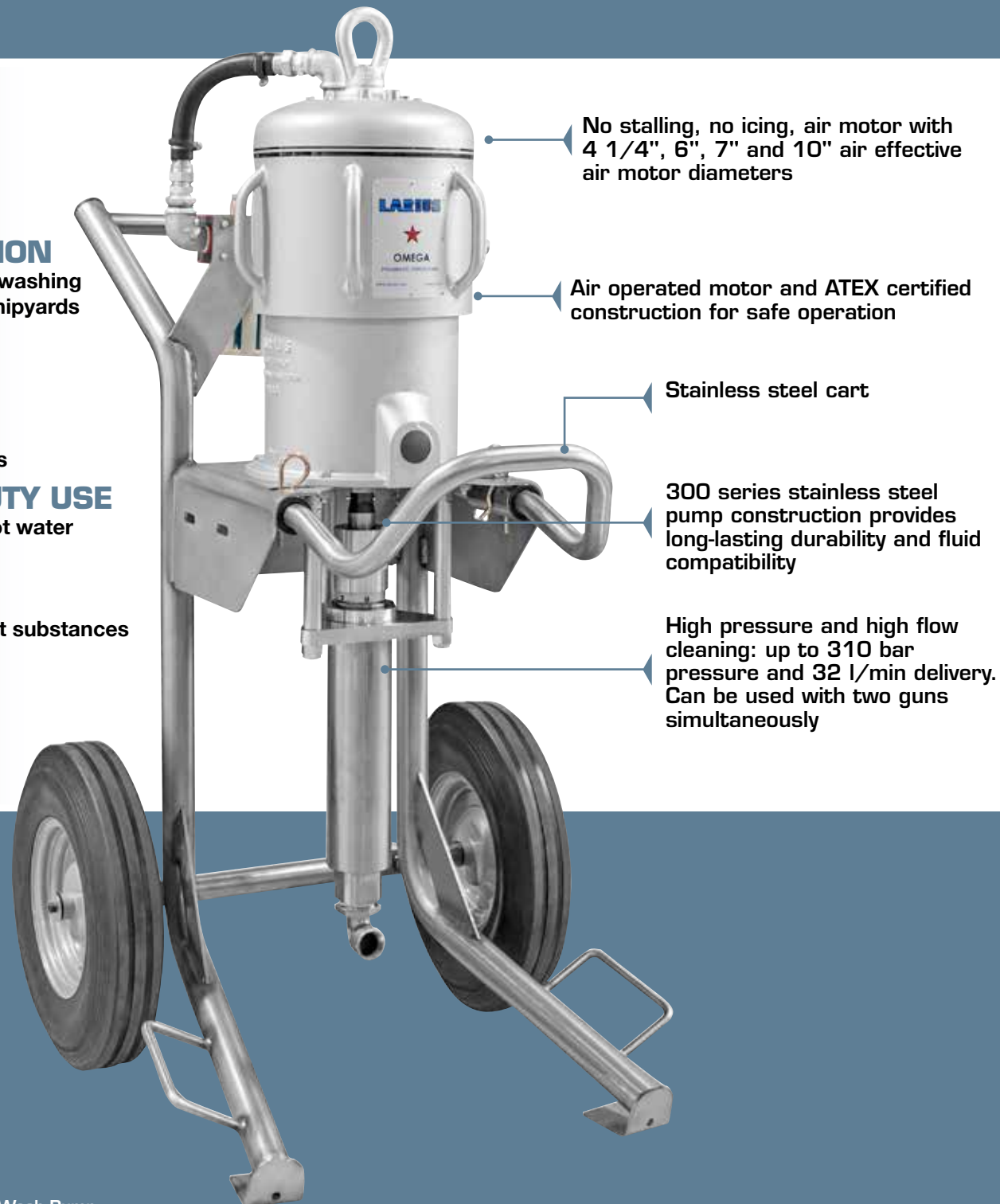
OMEGA Wash Pump
